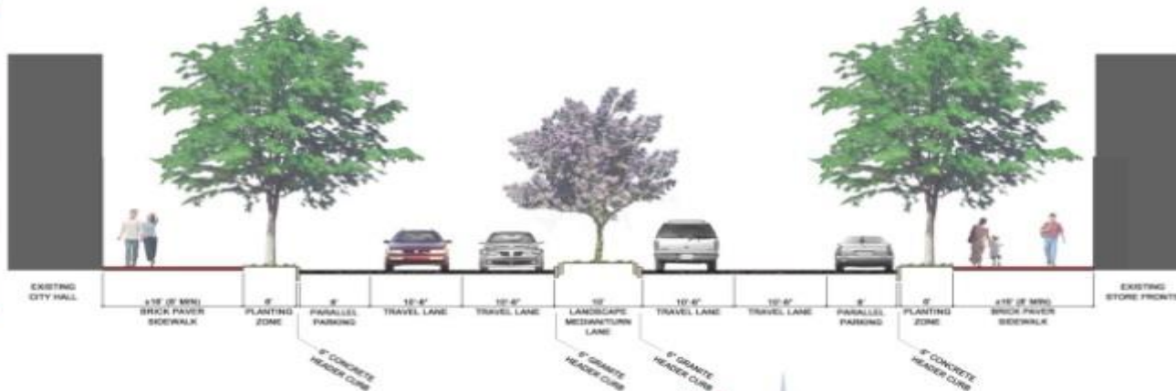
TYPICAL SECTION OF MAIN STREET IMPROVEMENTS
